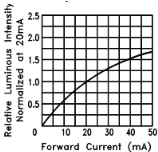
Fig.4 RELATIVE LUMINOUS INTENSITY VS. FORWARD CURRENT
