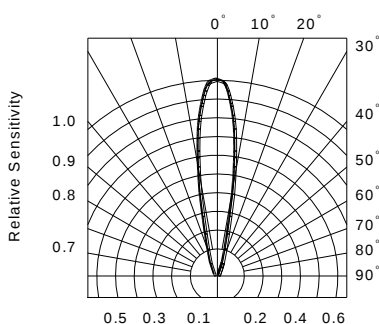
FIG.5 SENSITIVITY DIAGRAM
