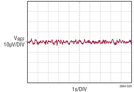
Reference 0.1Hz to 10Hz Voltage Noise
