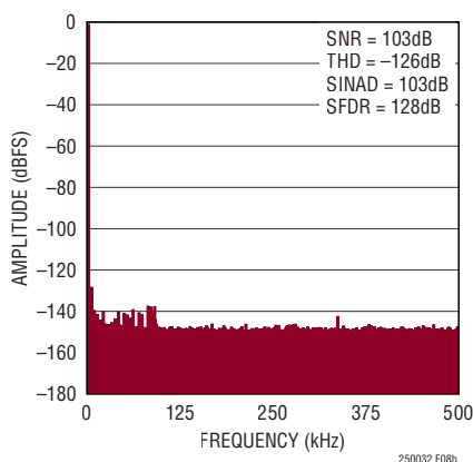
Figure 8b. 128k Point FFT Plot with F_{IN} = 2kHz for Circuit Shown in Figure 8a
