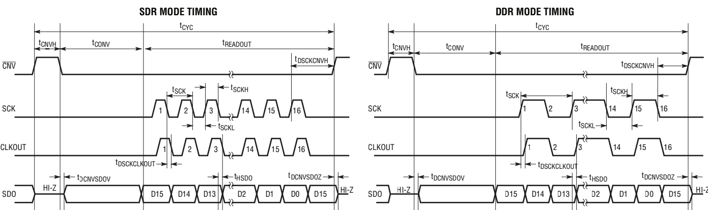
Figure 21. LTC2320-16 Timing Diagram
