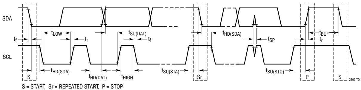
Definition of Timing for Fast/Standard Mode Devices on the I²C Bus
