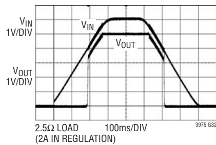
Start-Up/Dropout Performance
