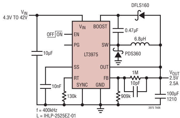
2.5V Step-Down Converter
