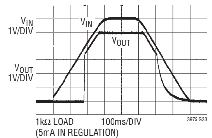
Start-Up/Dropout Performance
