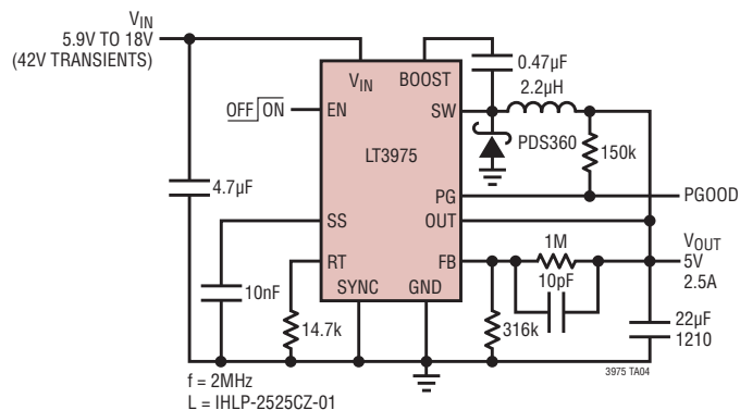
5V, 2MHz Step-Down Converter with Power Good
