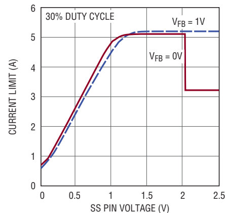
Soft-Start
