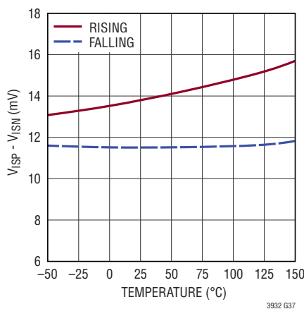
C/10 Threshold
