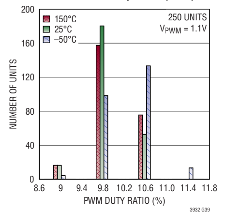
Internal PWM Duty Ratio (10%)
