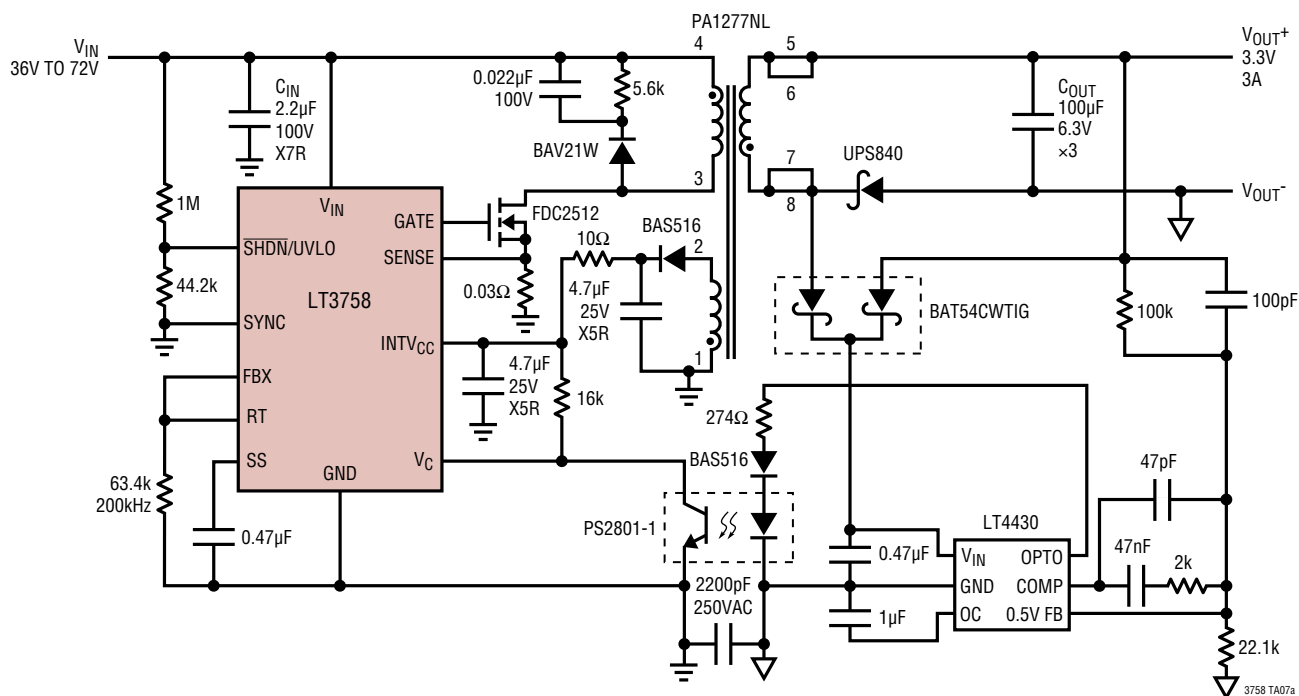
36V to 72V Input, 3.3V Output Isolated Telecom Power Supply
