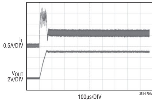
Figure 4a. Inductor Current Waveform During Start-Up without a Soft-Start Capacitor
