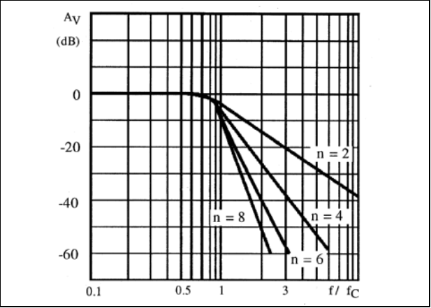
Figure 11. Amplitude response
