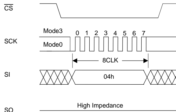
Figure 9 Write Disable
