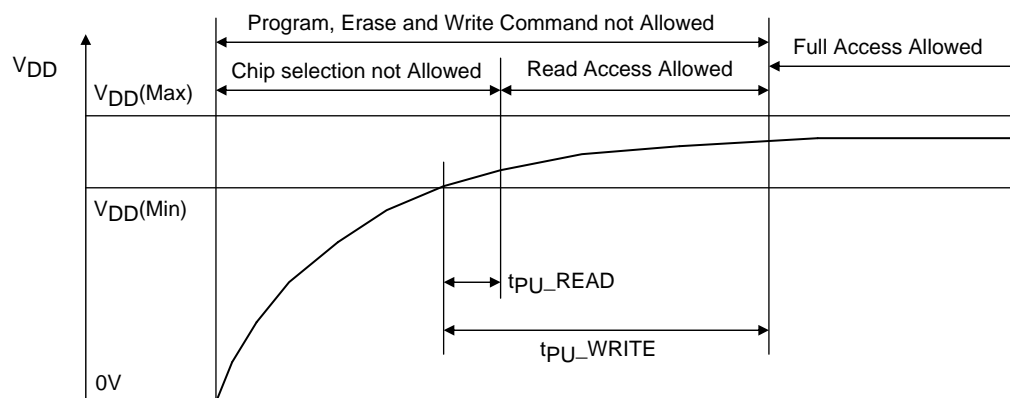
Figure 18 Power-on Timing
