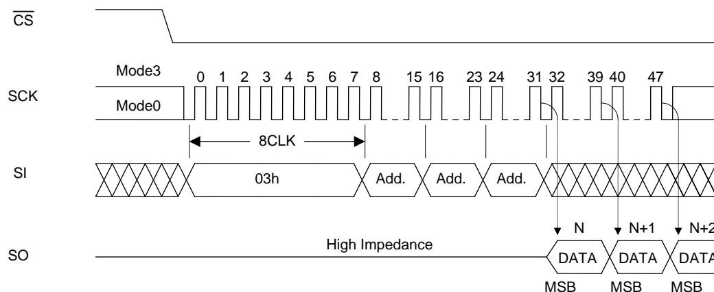
Figure 5-b 5 Bus Read
