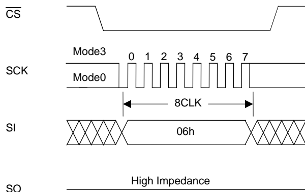
Figure 8 Write Enable
