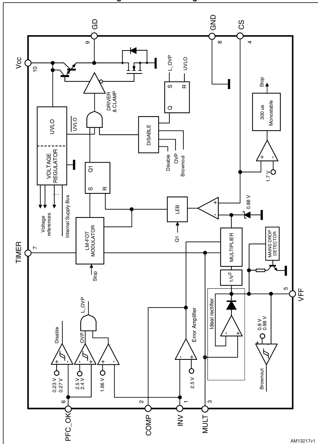
Figure 1. Electrical diagram
