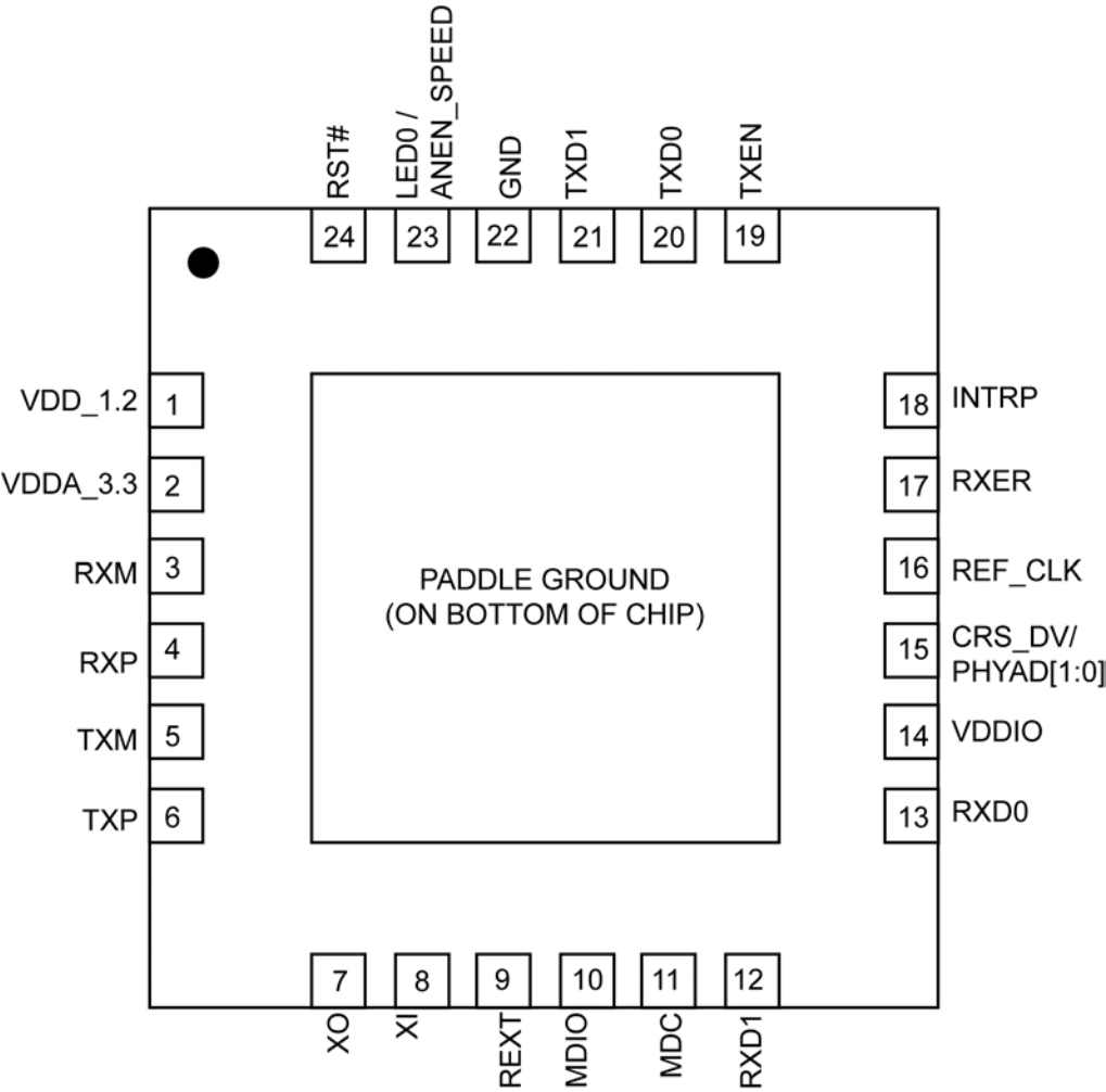
24-Pin 4mm x 4mm QFN
