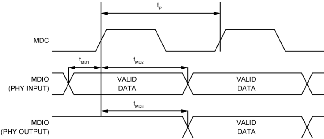
Figure 13. MDC/MDIO Timing
