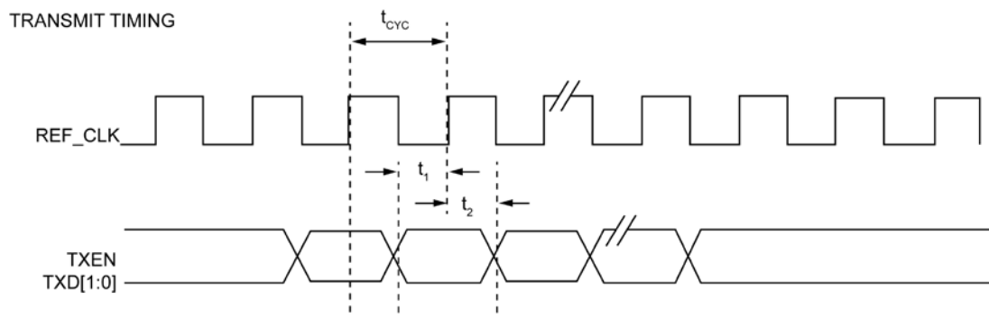
Figure 10. RMII Timing – Data Received from RMII
