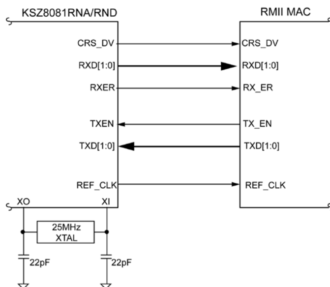
Figure 2. KSZ8081RNA/RND RMII Interface (RMII – 25MHz Clock Mode)
