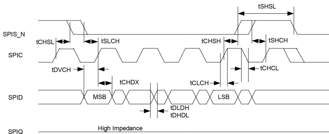
Figure 29. SPI Input Timing
