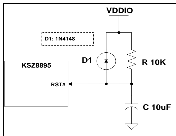
Figure 34. Recommended Reset Circuit
