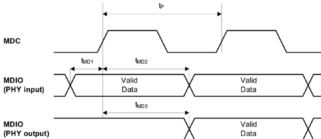
Figure 32. MDC/MDIO Timing
