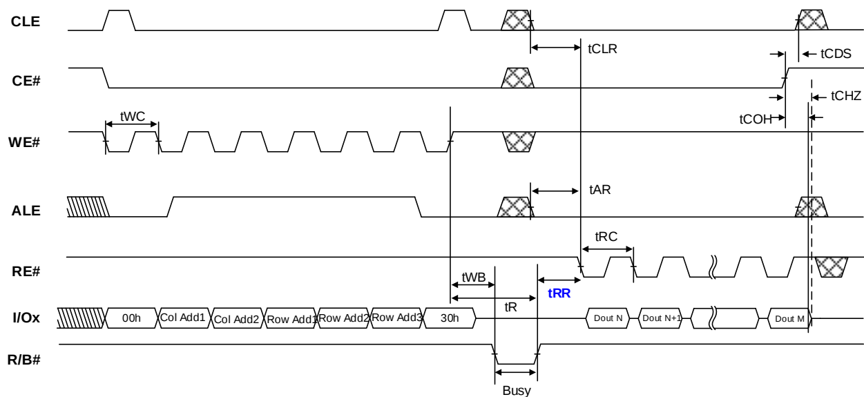
Figure 6.8 Read Operation (Intercepted by CE#)
