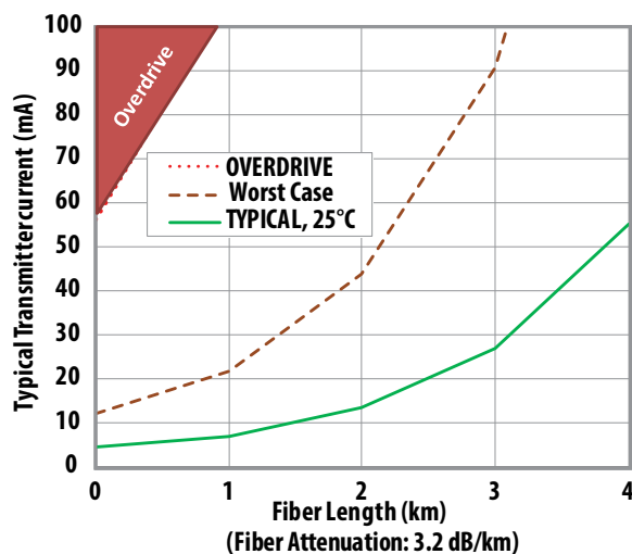
Figure 4: Typical HFBR-14x4xZ/HFBR-24x2xZ Link with 62.5/125 \mu\text{m} Fiber
