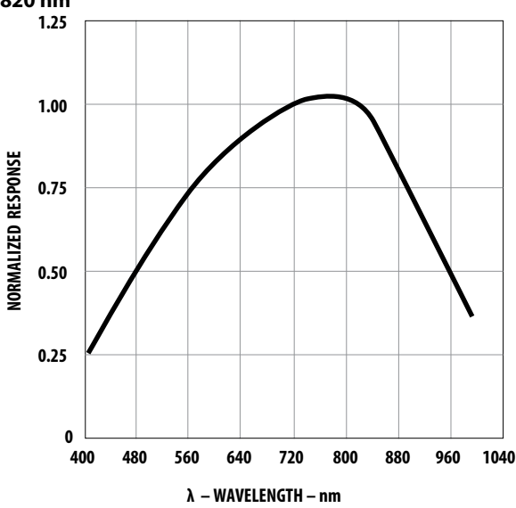
Figure 18: Typical Receiver Spectral Response Normalized to 820 nm
