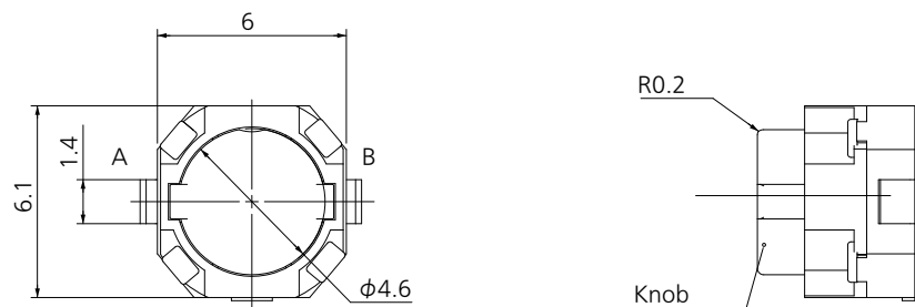
CAD External dimensions
