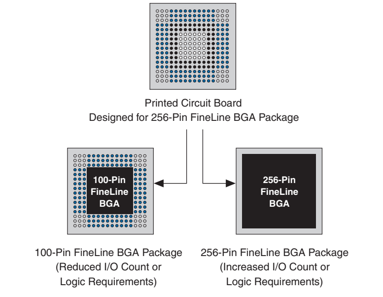
Figure 15. SameFrame Pin-Out Example
