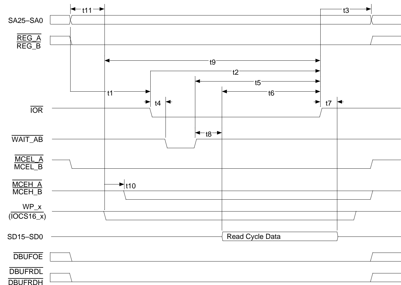
Figure 59. PC Card I/O Read Cycle
