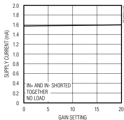
SUPPLY CURRENT vs. GAIN SETTING
