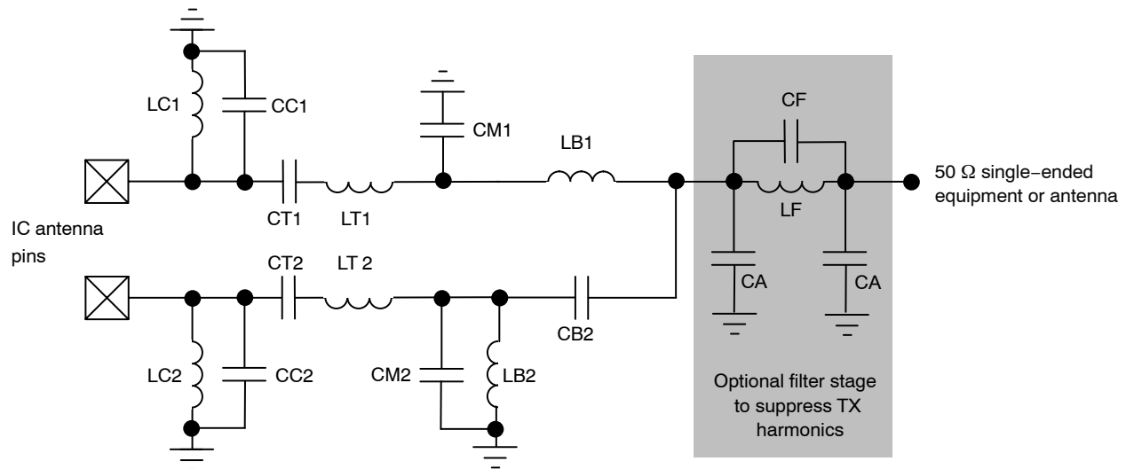
Figure 9. Structure of the Differential Antenna Interface for TX/RX Operation to 50 \Omega Single-ended Equipment or Antenna
