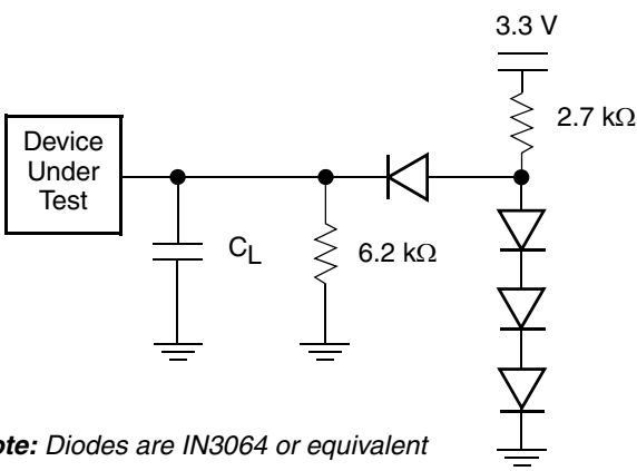
Figure 11. Test Setup
