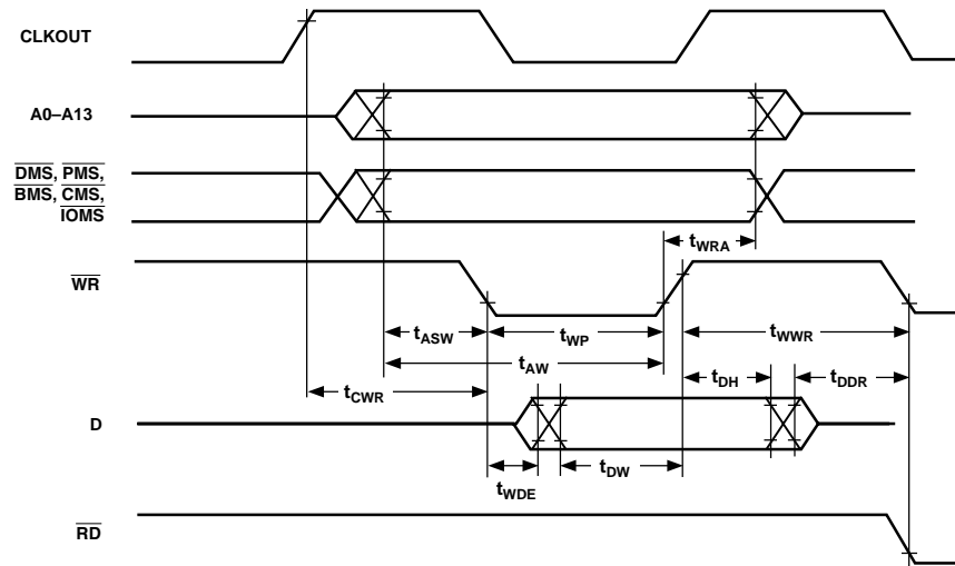
Figure 19. Memory Write
