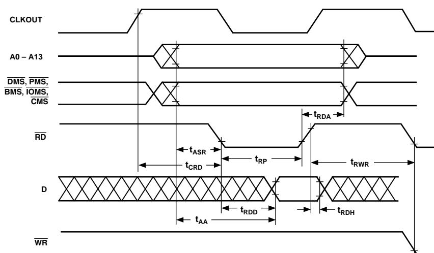
Figure 18. Memory Read
