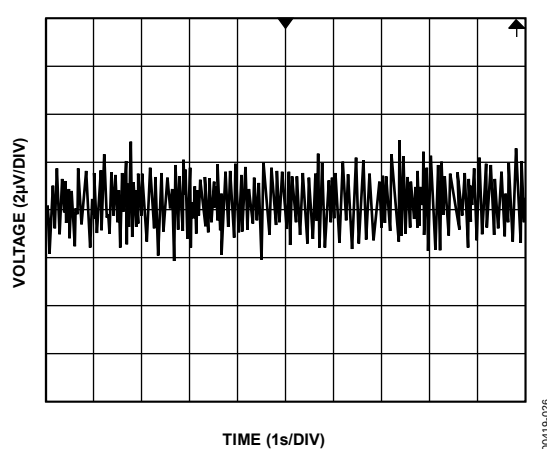
Figure 25. ADR391 Typical Voltage Noise 0.1 Hz to 10 Hz
