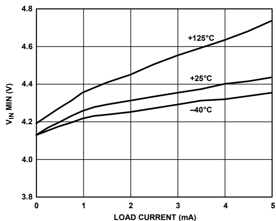
Figure 20. ADR392 Minimum Input Voltage vs. Load Current
