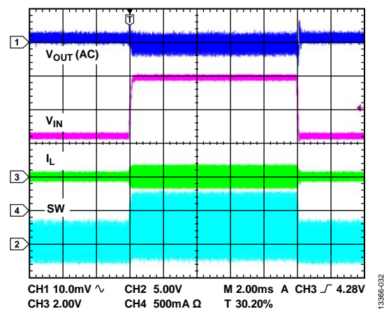
Figure 32. Line Transient of PWM Mode, I_{LOAD} = 500 \mu A ( I_L is the Inductor Current)
