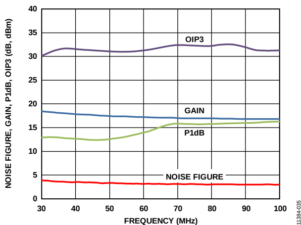
Figure 36. Noise Figure, Gain, P1dB, and OIP3 vs. Frequency, 30 MHz to 100 MHz
