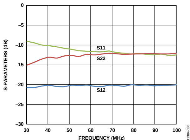
Figure 37. Return Loss and Reverse Isolation, 30 MHz to 100 MHz
