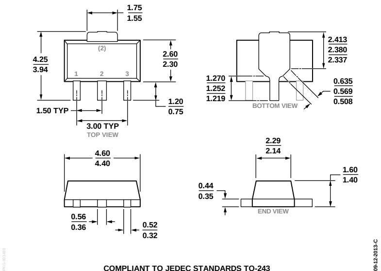
COMPLIANT TO JEDEC STANDARDS TO-243 Figure 42. 3-Lead Small Outline Transistor Package [SOT-89] (RK-3) Dimensions shown in millimeters
