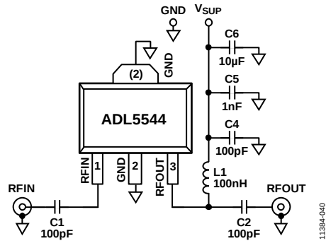
Figure 41. Evaluation Board Schematic
