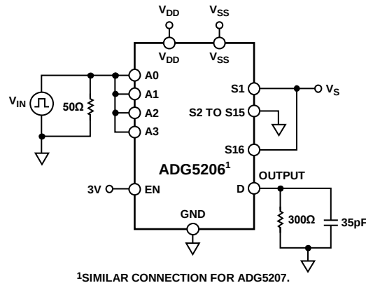
Figure 37. Break-Before-Make Time Delay, t_D
