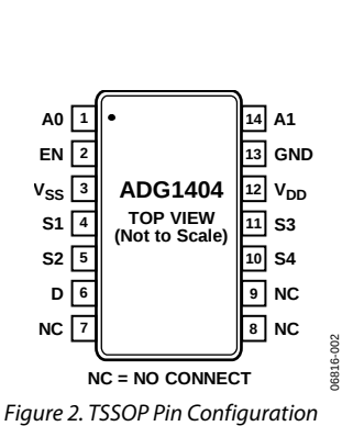
Figure 2. TSSOP Pin Configuration
