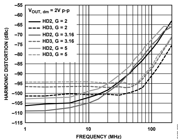
Figure 17. Harmonic Distortion vs. Frequency at Various Gains
