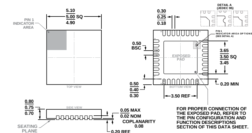
Figure 55. 32-Lead Lead Frame Chip Scale Package [LFCSP] 5 mm × 5 mm Body and 0.75 mm Package Height (CP-32-11)
