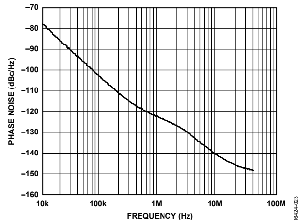
Figure 28. Internal VCO Phase Noise (Absolute) Direct to LVPECL at 2950 MHz
