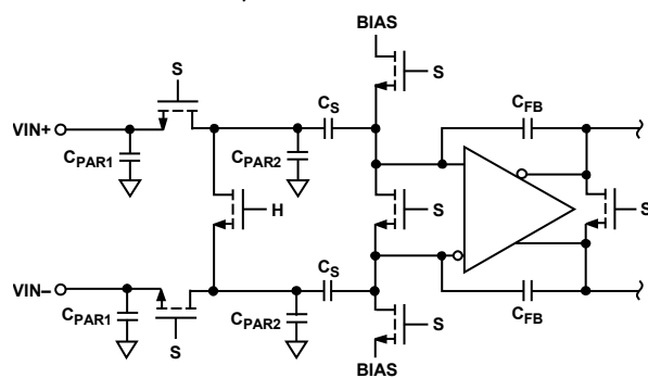
Figure 64. Switched Capacitor Input
