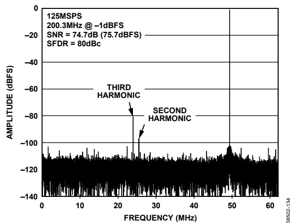
Figure 34. AD9265-125 Single-Tone FFT with f_{IN} = 200.3 MHz
