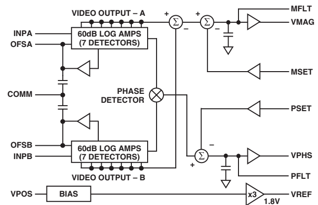
Figure 2. General Structure
