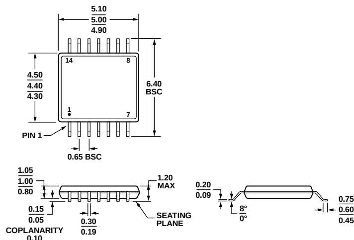
Figure 18. 14-Lead Thin Shrink Small Outline Package [TSSOP] (RU-14) Dimensions shown in millimeters
