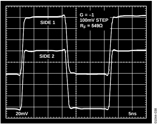
Figure 39. 100 mV Step Response, G = -1
