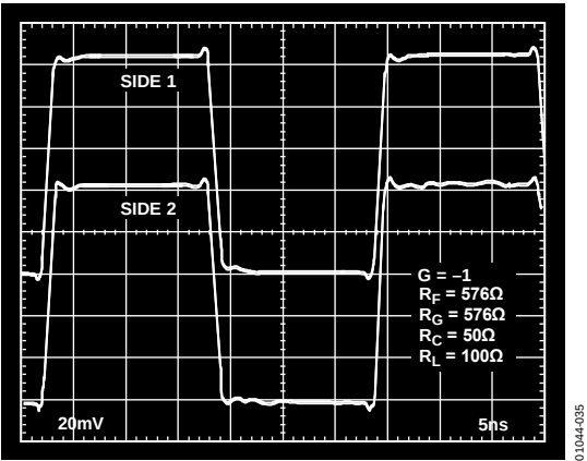
Figure 36. 100 mV Step Response, G = -1
