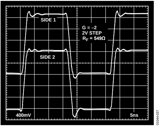
Figure 38. 2 V Step Response, G = -2
