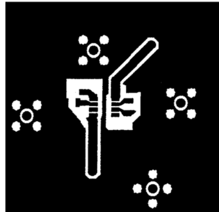
Figure 69. Noninverter SOIC Board Layout (Solder Side) (Looking Through the Board)
