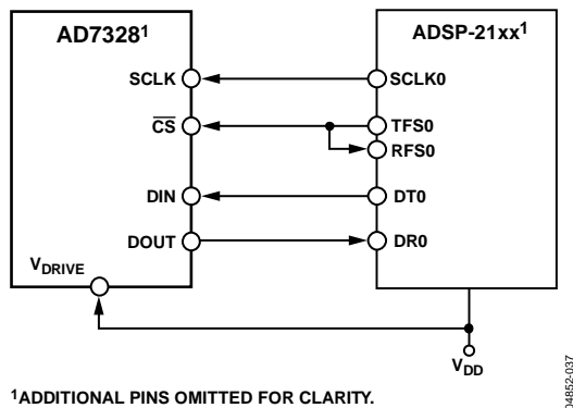
Figure 54. Interfacing the AD7328 to the ADSP-21xx
