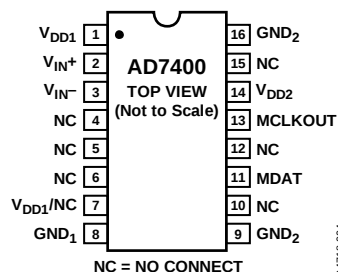
Figure 5. Pin Configuration
