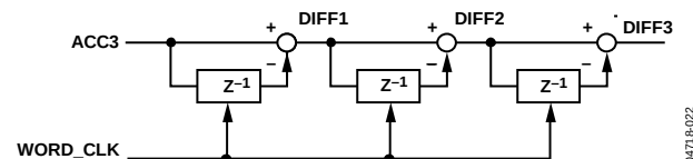
Figure 26. Differentiator
