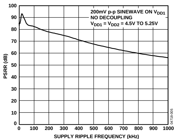
Figure 6. PSRR vs. Supply Ripple Frequency Without Supply Decoupling (1 MHz Filter Used)
