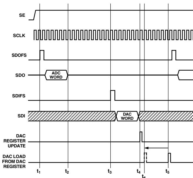
Figure 39. DAC Timing Control
