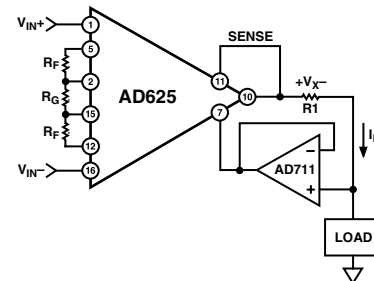
Figure 31. Voltage-to-Current Converter
