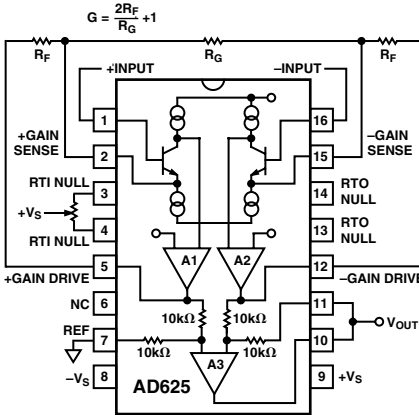
Figure 27. AD625 in Fixed Gain Configuration
