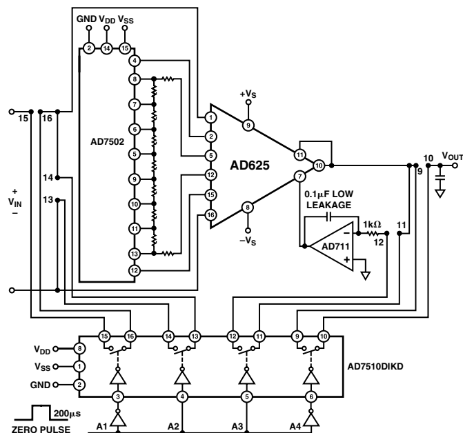
Figure 36. Auto-Zero Circuit
