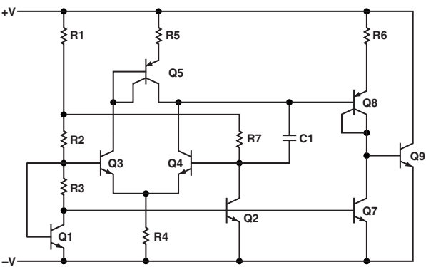
Figure 4. Schematic Diagram
