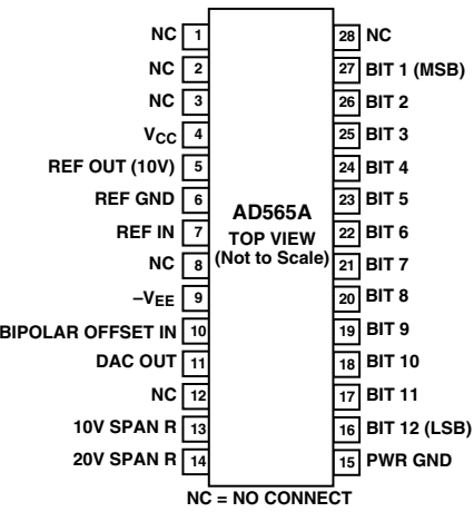
28-Lead SOIC
