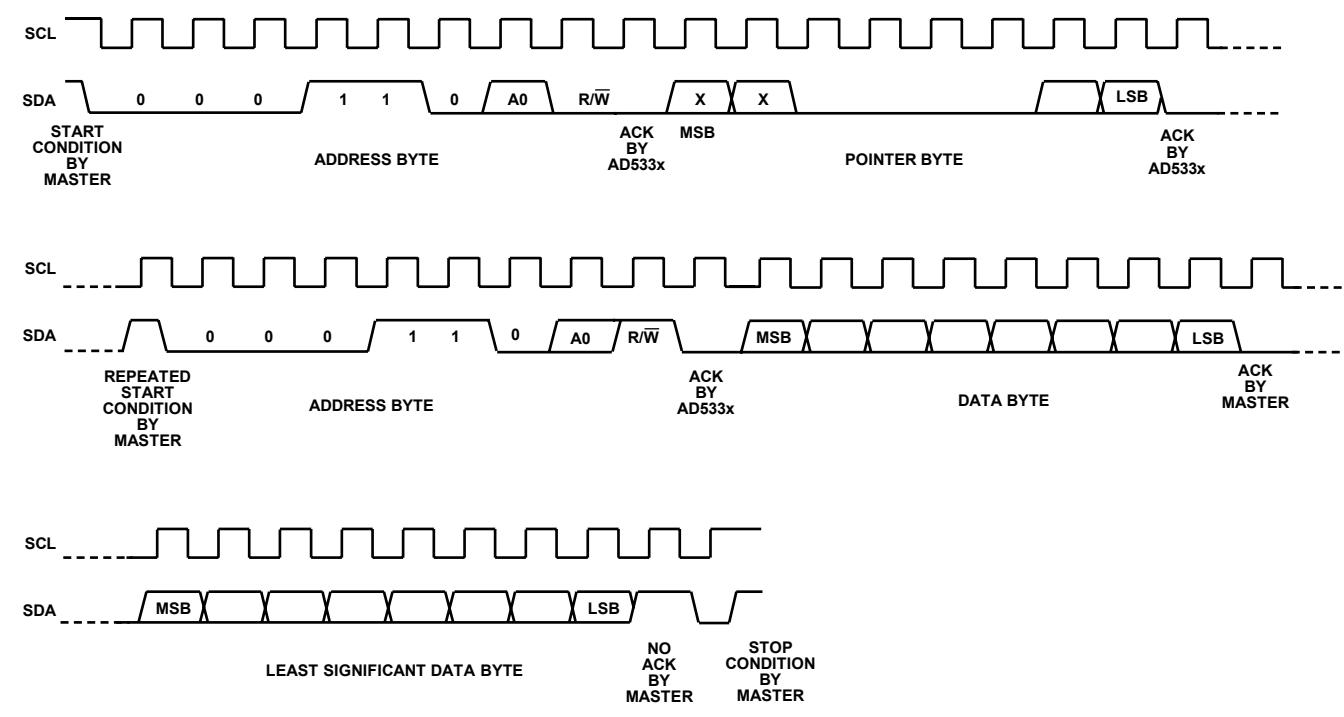
Figure 34. Read Sequence
