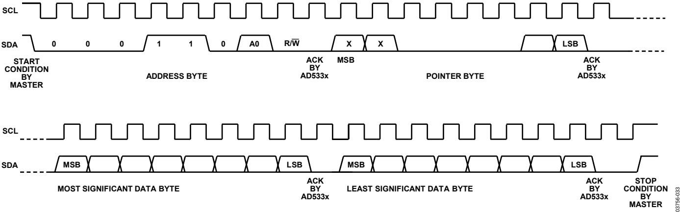
Figure 33. Write Sequence
