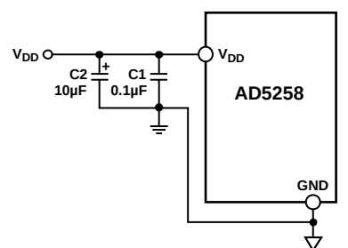
Figure 42. Power Supply Bypassing
