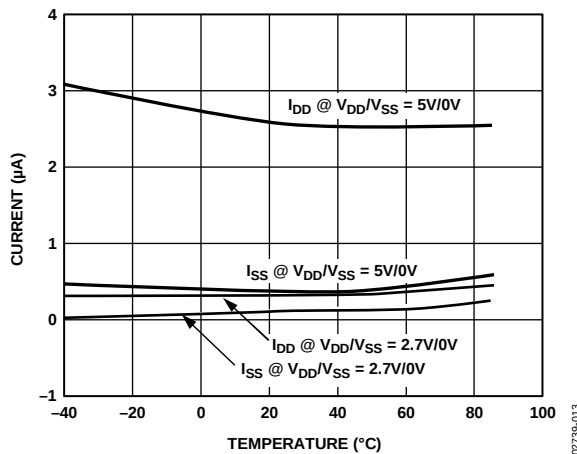
Figure 13. I_{DD} vs. Temperature, R_{AB} = 10\text{ k}\Omega
