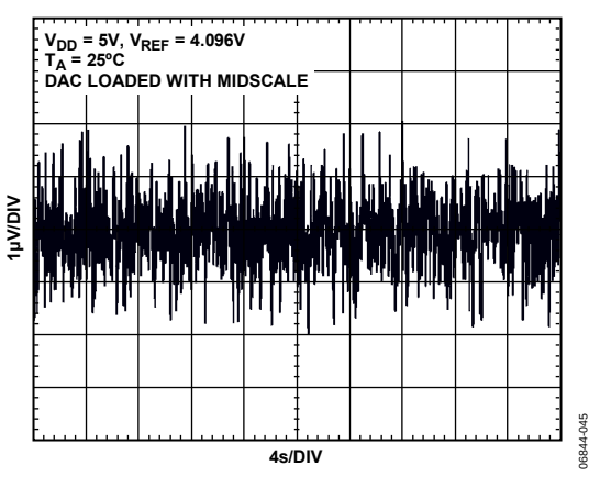
Figure 28. 0.1 Hz to 10 Hz Output Noise Plot
