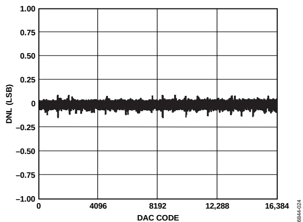
Figure 11. AD5025 DNL
