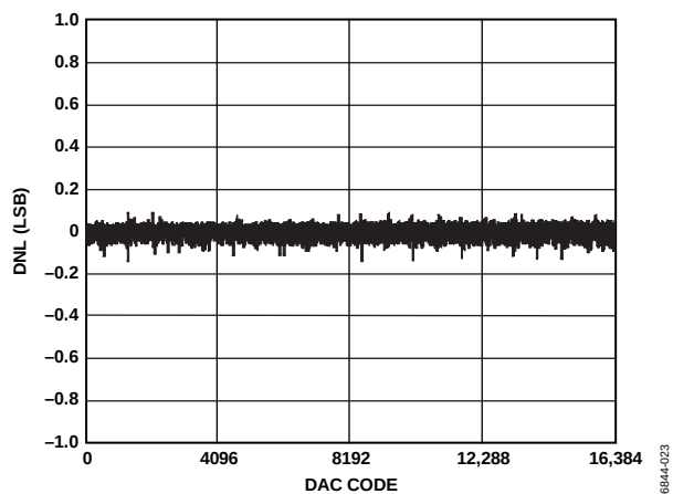
Figure 10. AD5045 DNL
