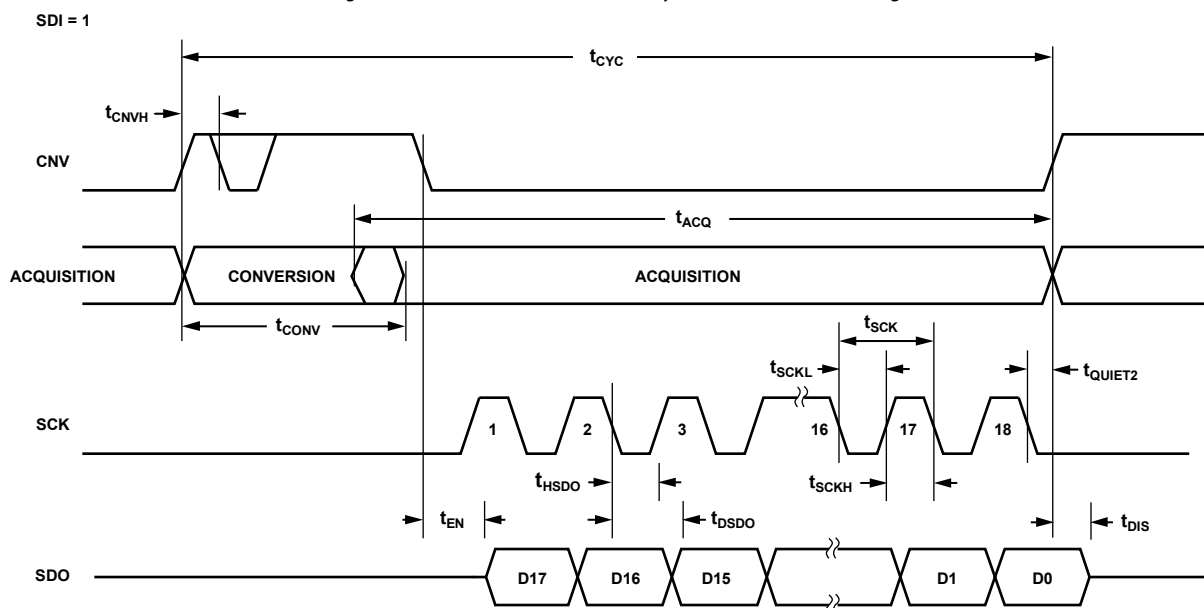
Figure 56. \overline{\text{CS}} Mode, 3-Wire Without Busy Indicator Serial Interface Timing Diagram (Status Bits Not Shown)
