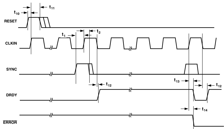
Figure 4. AD1556 RESET, DRDY, and Overwrite Timings
