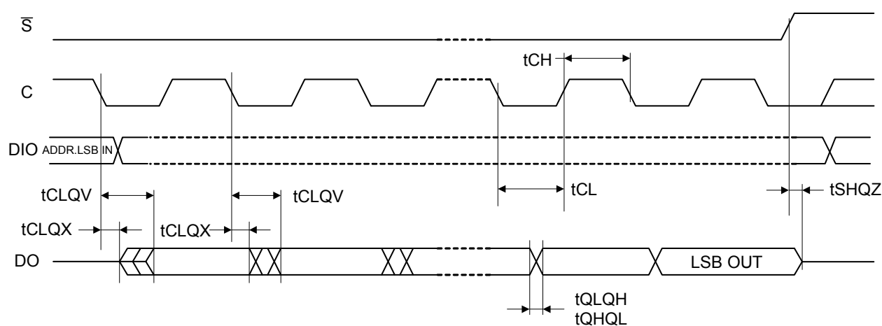
Figure 26. Output Timing
