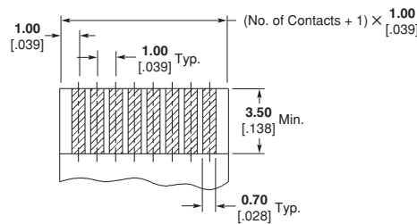
Recommended FPC Layout
