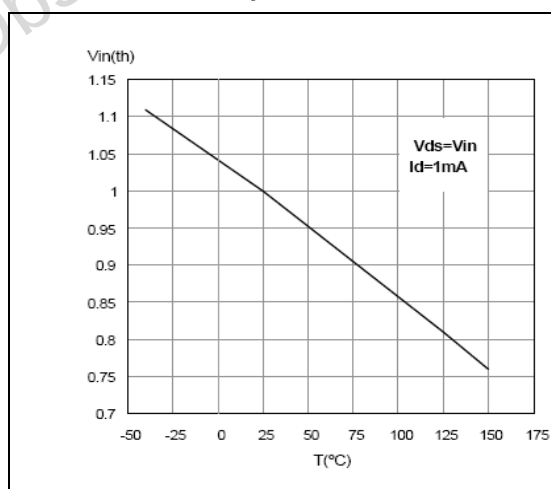
Figure 39. Normalized input threshold voltage vs temperature
