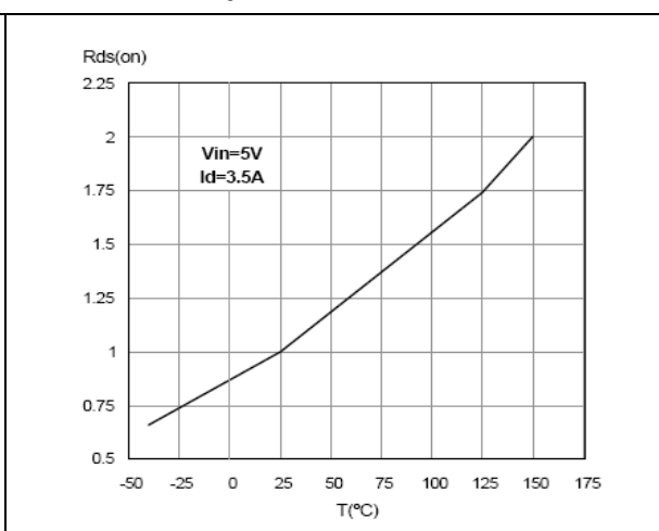
Figure 40. Normalized on resistance vs temperature
