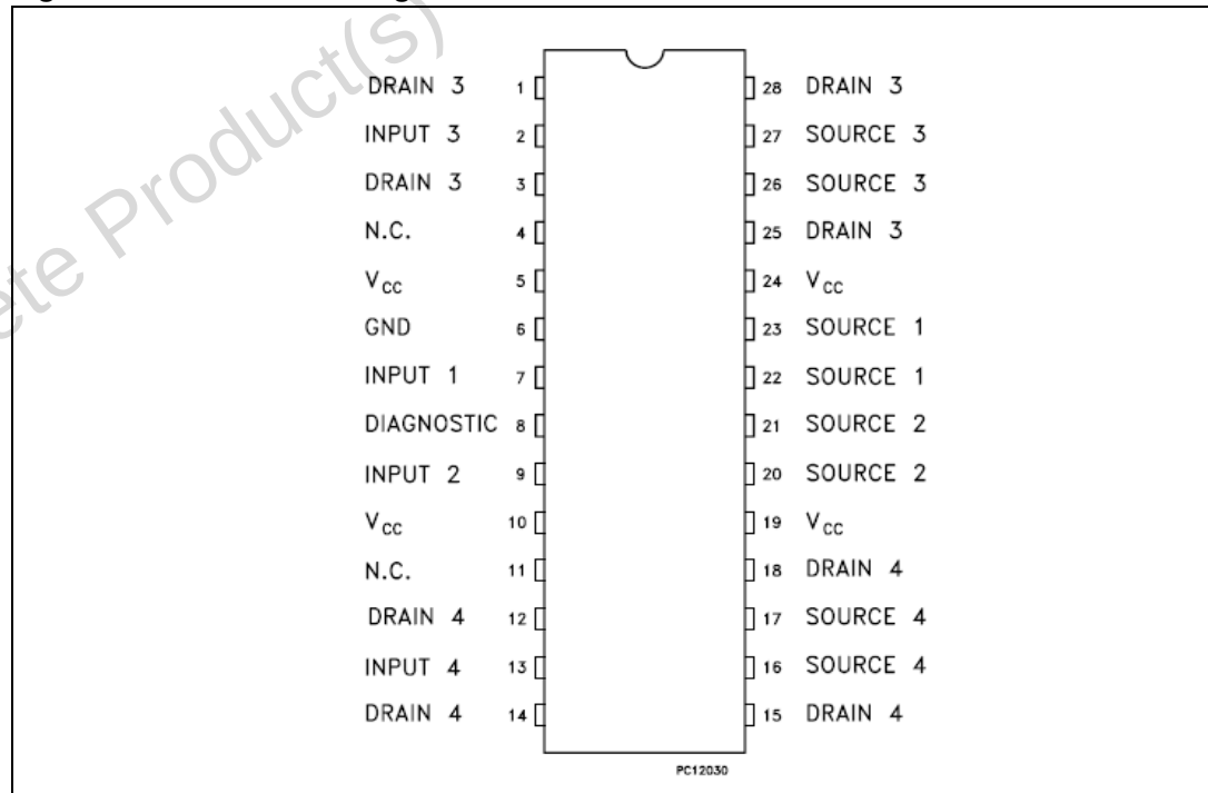
Figure 2. Connection diagram
